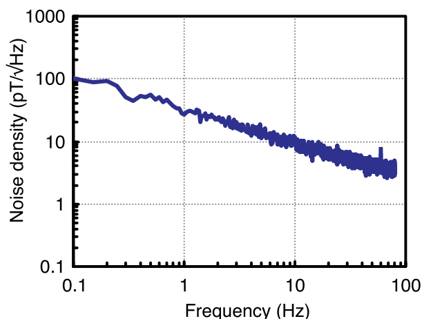
Fig. Noise spectrum
